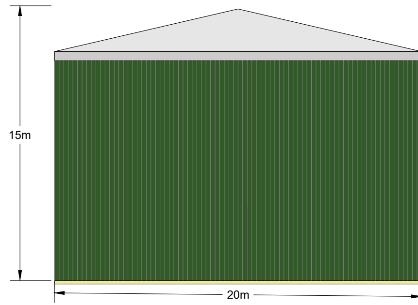
North Elevation
